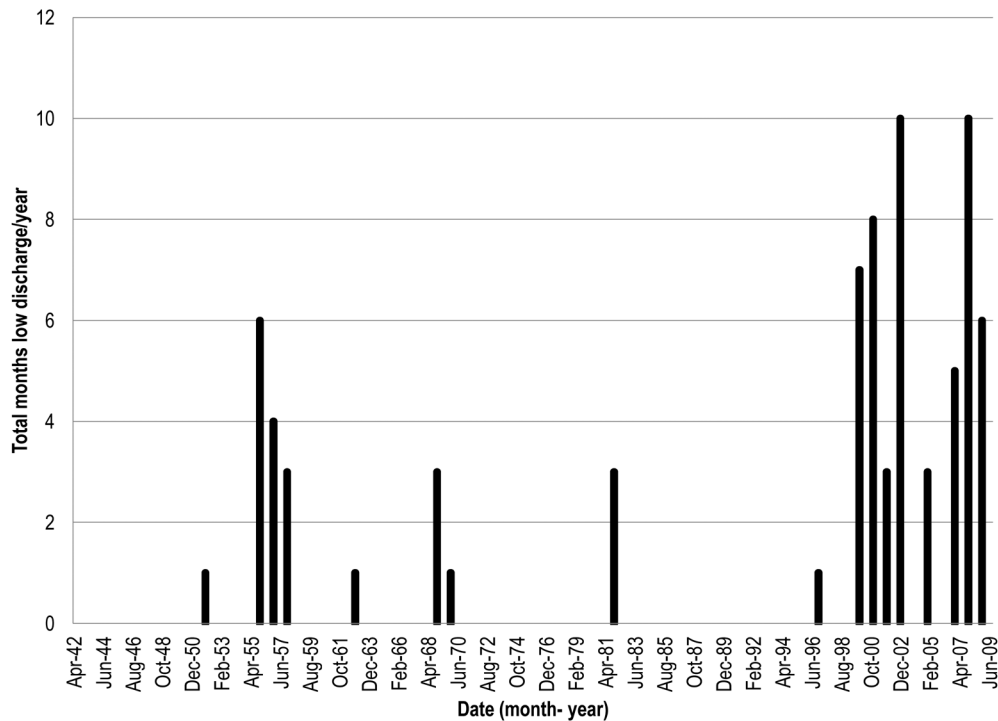
Fig. 7. Number of months low discharge (<1 SD below period of record monthly mean) from the Suwannee River, 1942–2009.
